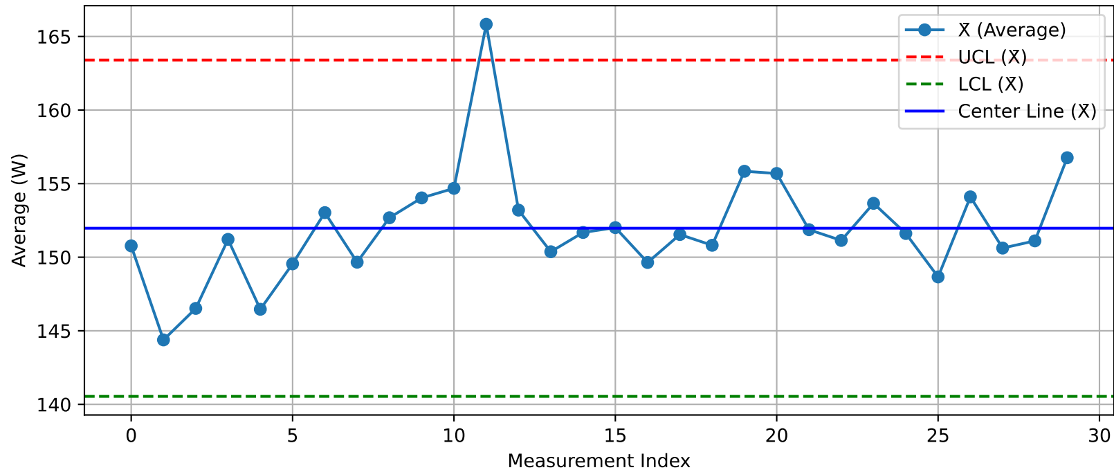
DUT - \bar{X} Chart (T51@Test1_Nuitka.xlsx)
