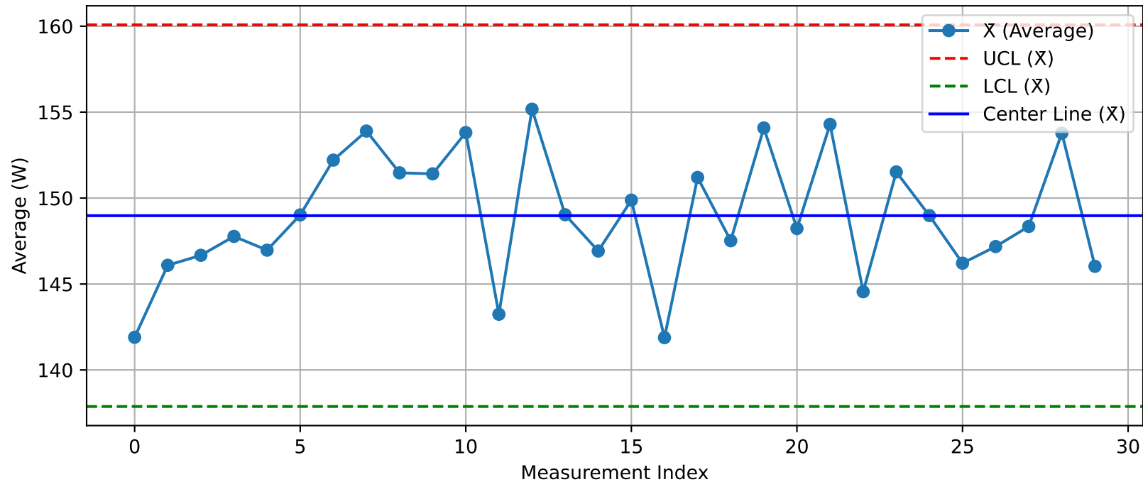
DUT - \bar{X} Chart (T51@Test2_Nuitka.xlsx)
