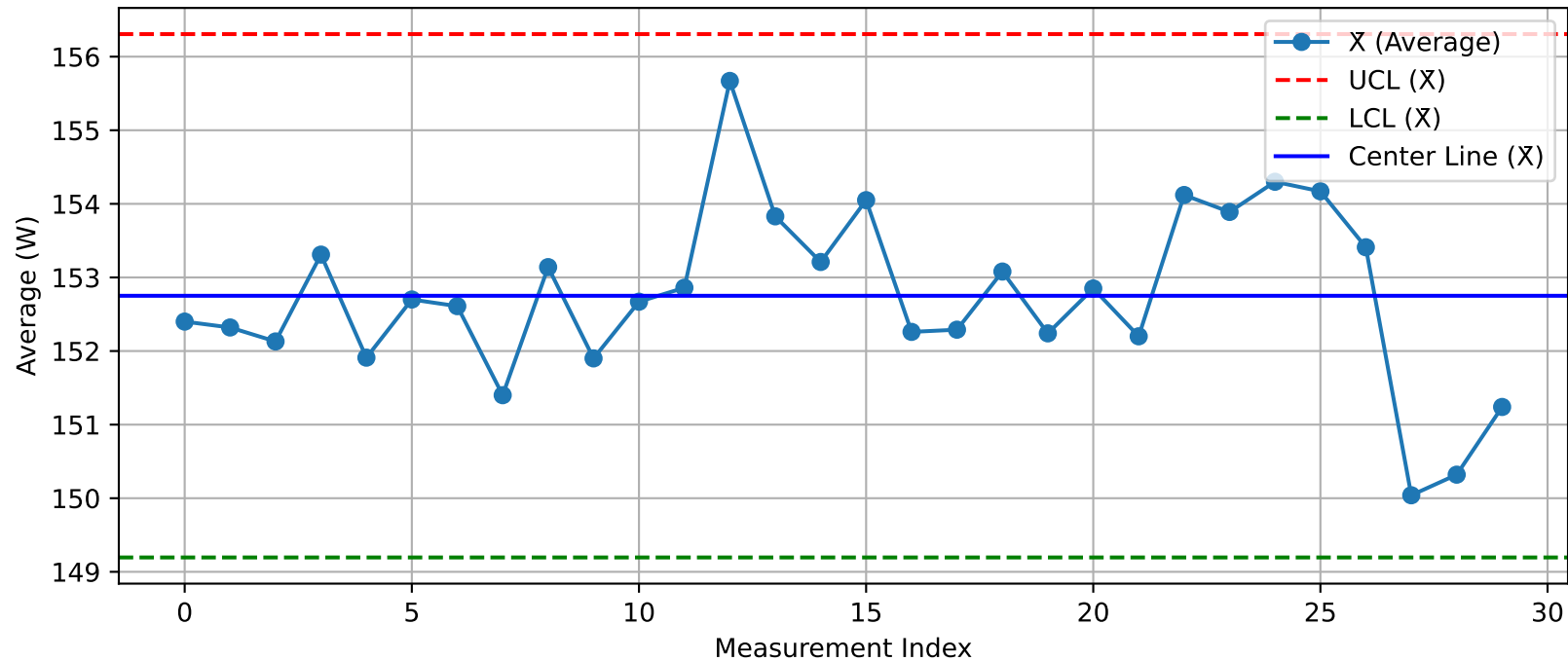
DUT - \bar{X} Chart (T5@Test1_Nuitka.xlsx)
