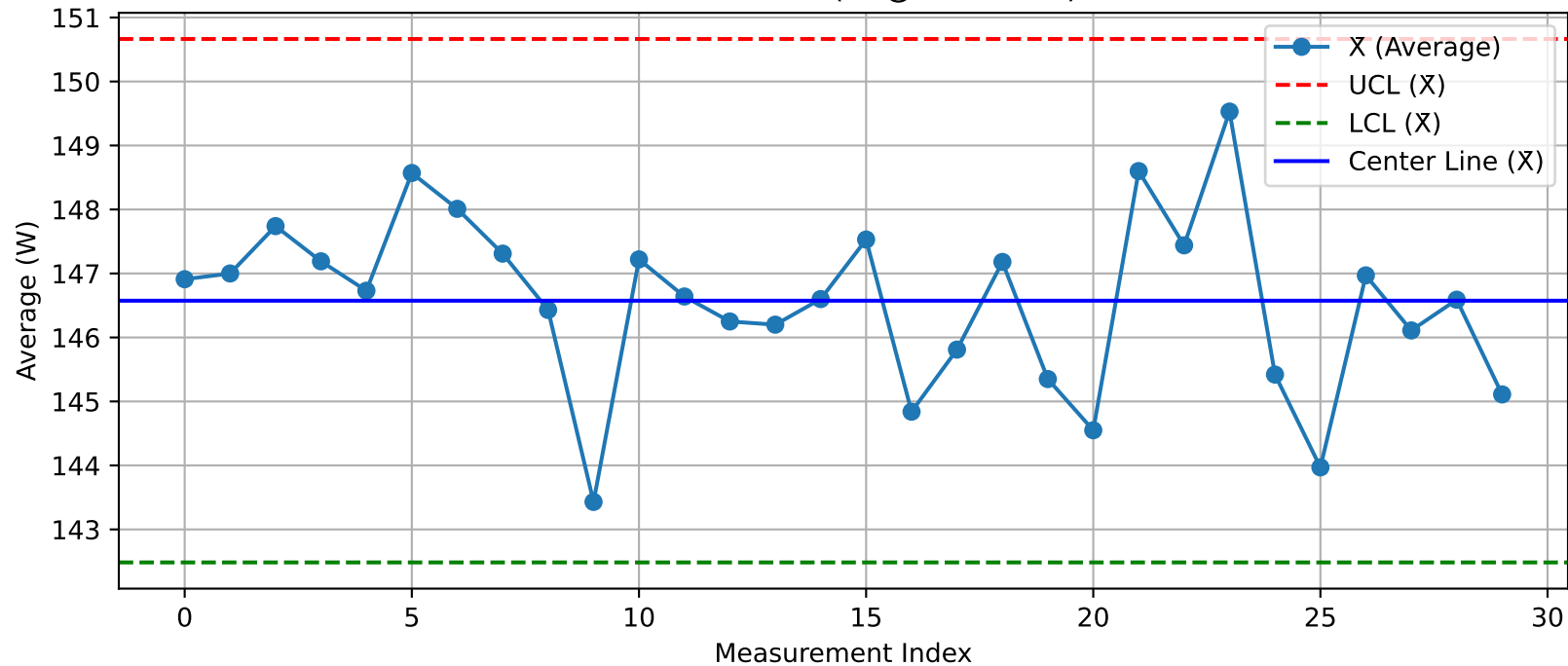
DUT - \bar{X} Chart (T5@Test2.xlsx)
