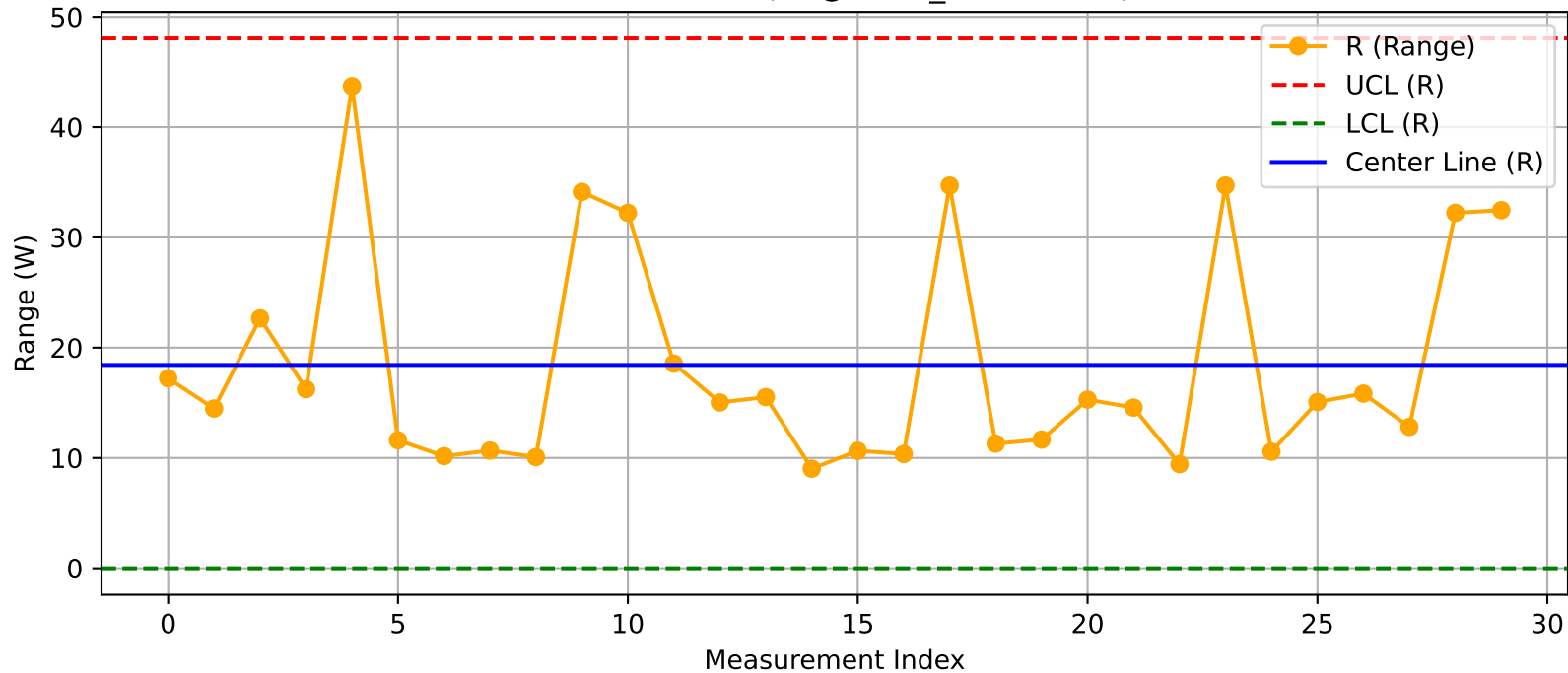
DUT - R Chart (T7@Test1_Nuitka.xlsx)
