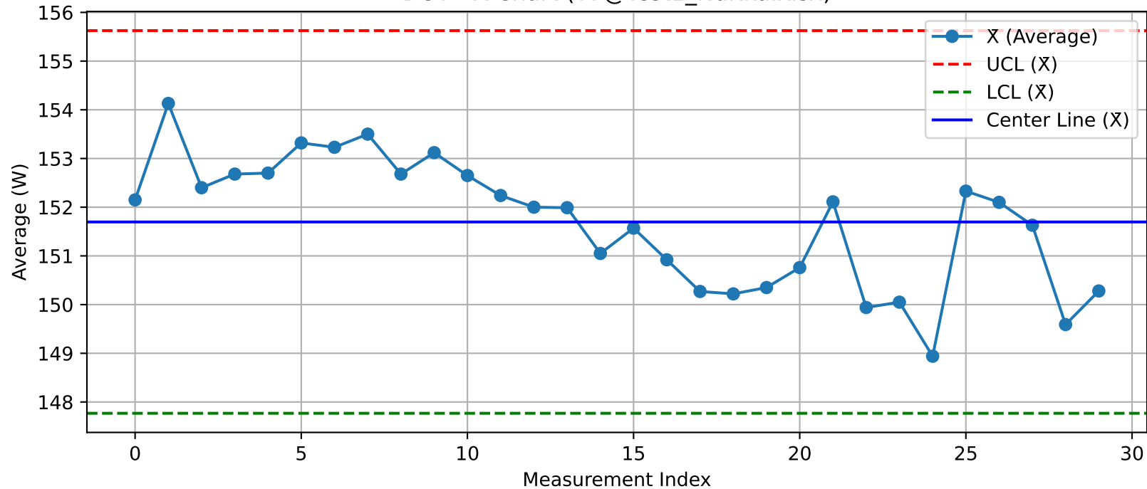
DUT - \bar{X} Chart (T7@Test1_Nuitka.xlsx)
