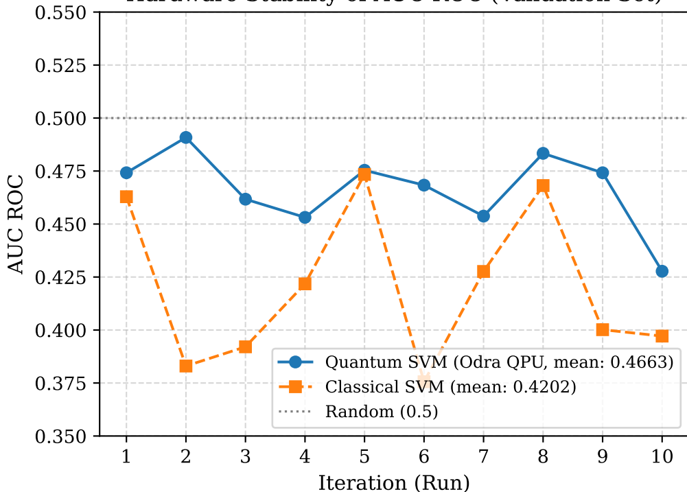
Hardware Stability of AUC ROC (Validation Set)
