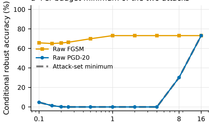
a Per-budget minimum of the two attacks
