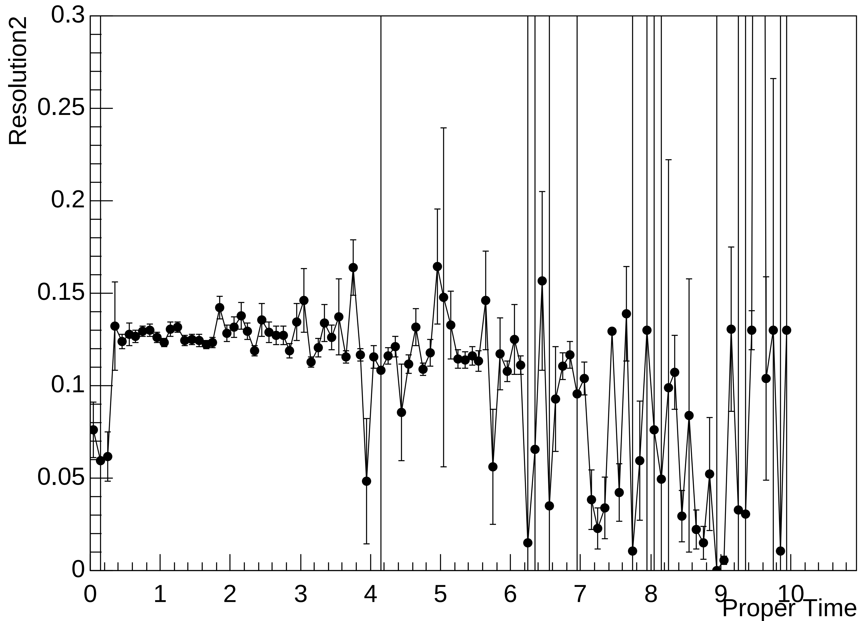
Resolution2 vs Proper Time
