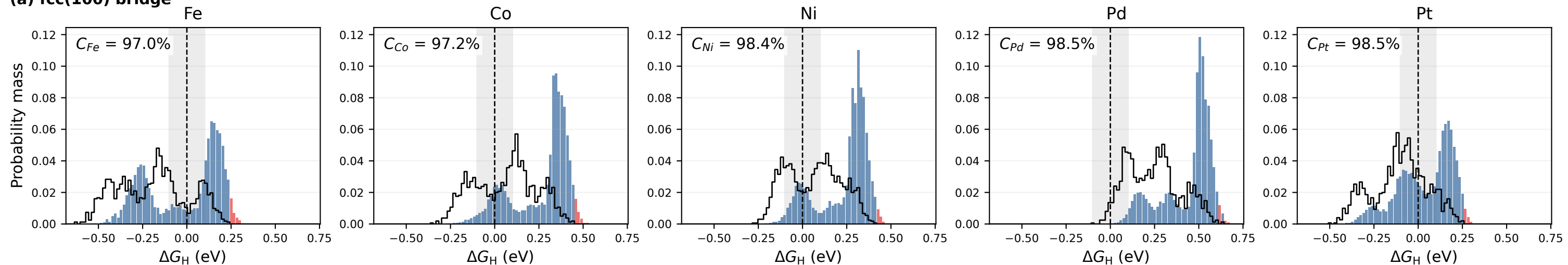
(a) fcc(100) bridge
