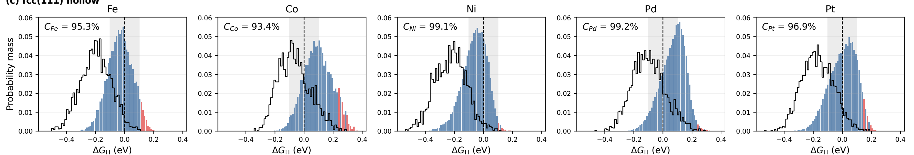
(c) fcc(111) hollow
