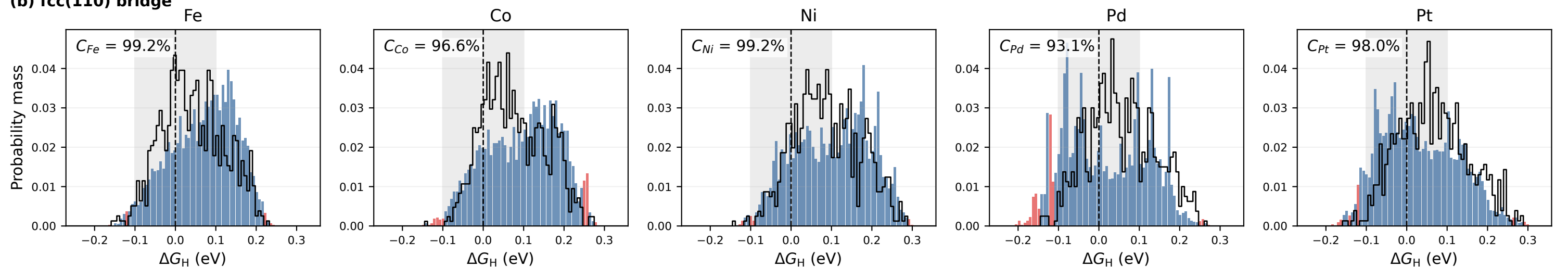
(b) fcc(110) bridge
