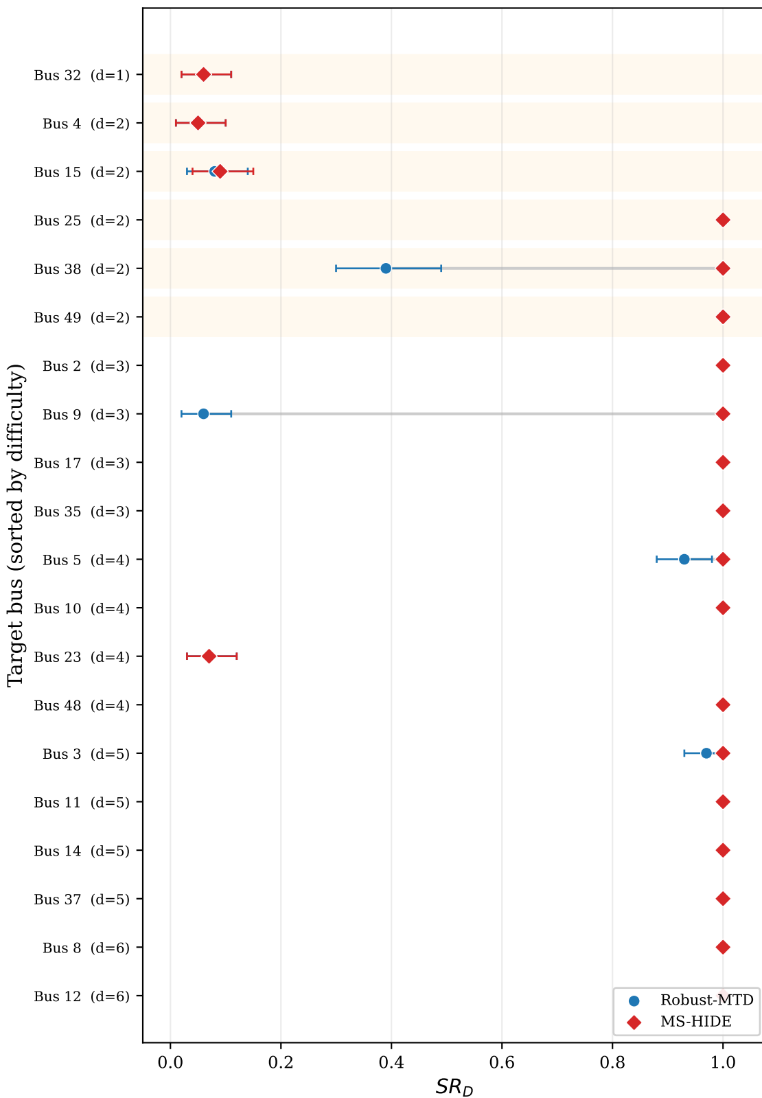
(a) Detection success rate SR_D
