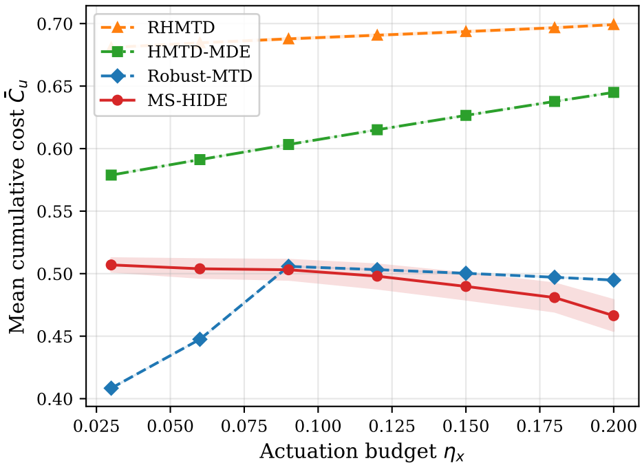
(b) Actuation cost vs. \eta_x
