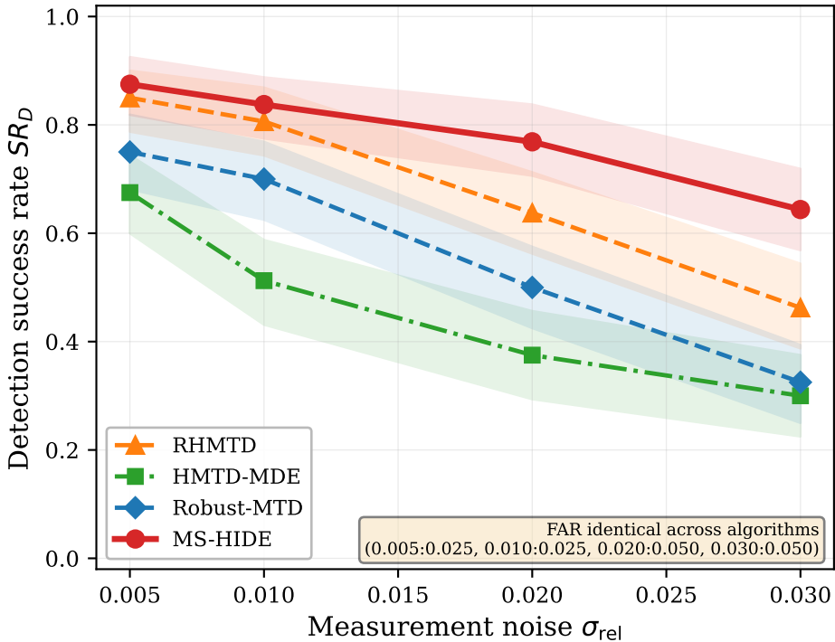
(a) Detection rate vs. \sigma_{\text{rel}}
