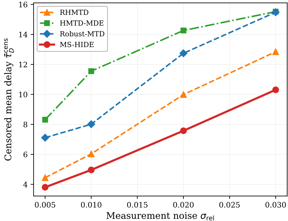
(b) Detection delay vs. \sigma_{\text{rel}}
