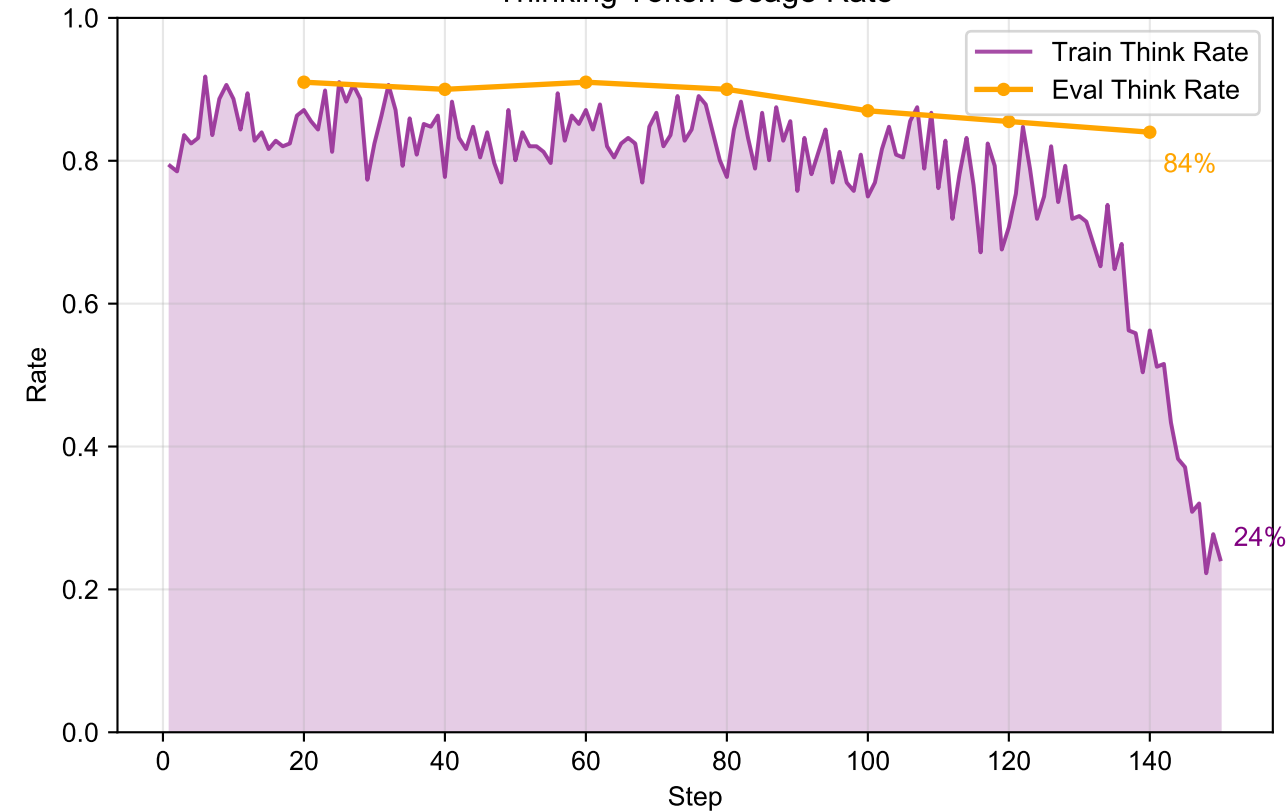
Thinking Token Usage Rate
