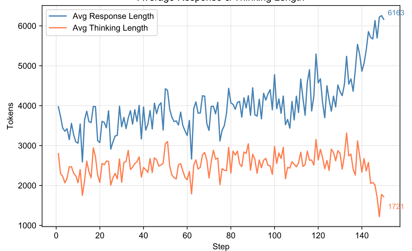
Average Response & Thinking Length
