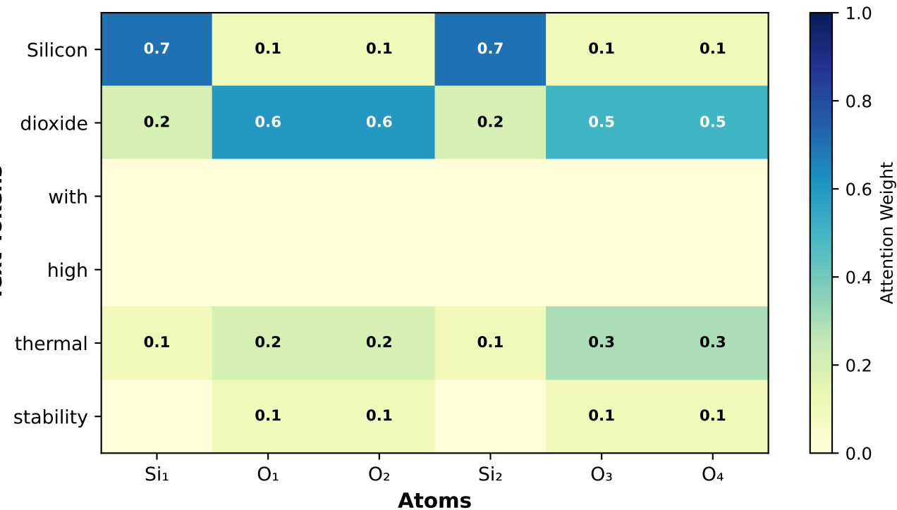
Token-to-Atom Attention (Which atoms does each word attend to?)
