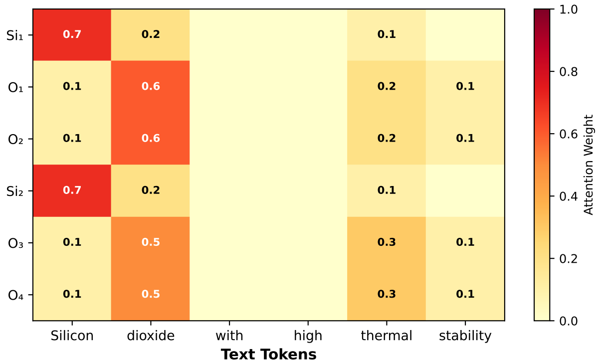
Atom-to-Token Attention (Which words does each atom attend to?)
