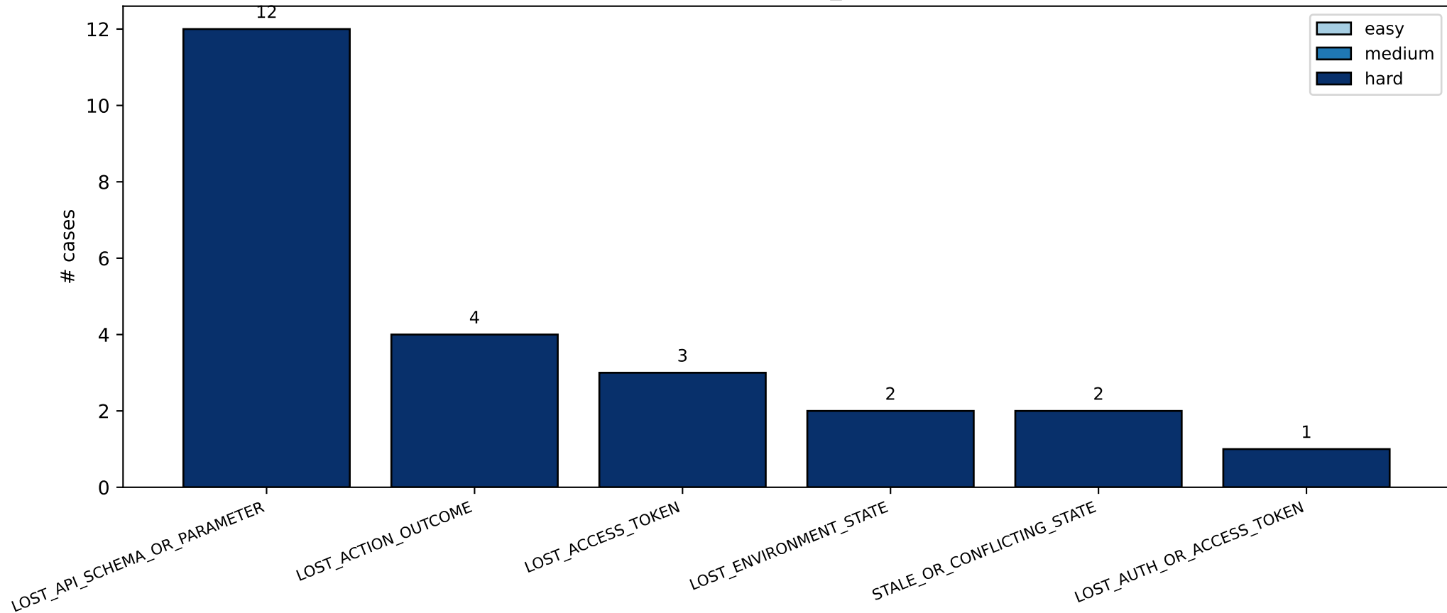
ACON failure-mode distribution (n_cases per primary mode)
