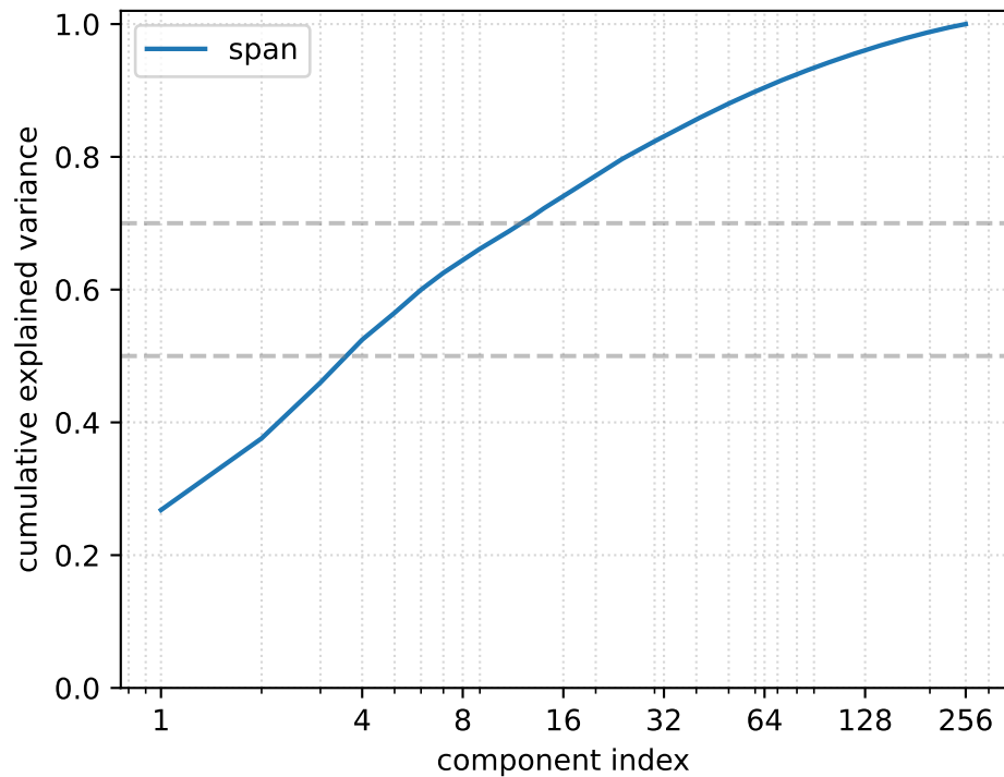
Span-level active subspace spectrum (layer 18)
