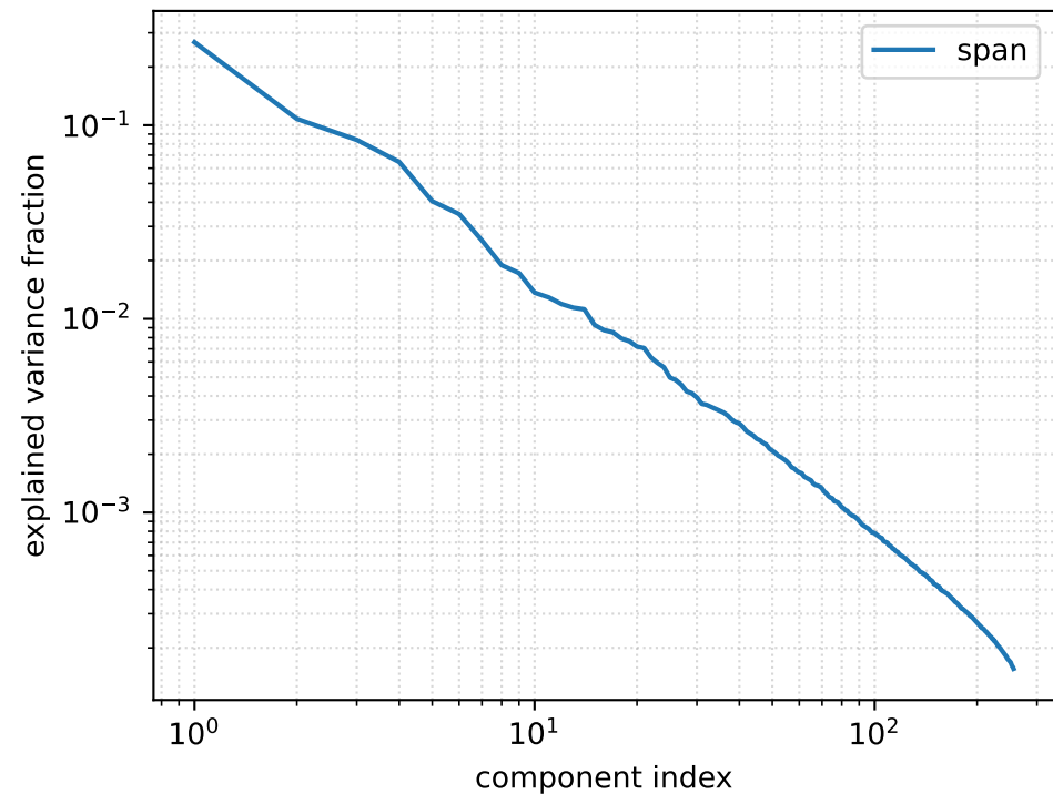
Span-level active subspace spectrum (layer 18)
