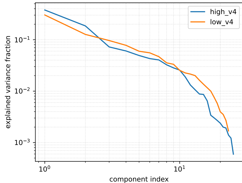
High vs low v4-sensitivity spans (layer 18)
