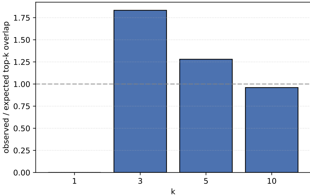
Top-k overlap enrichment (Jacobian n v4-sensitivity)
