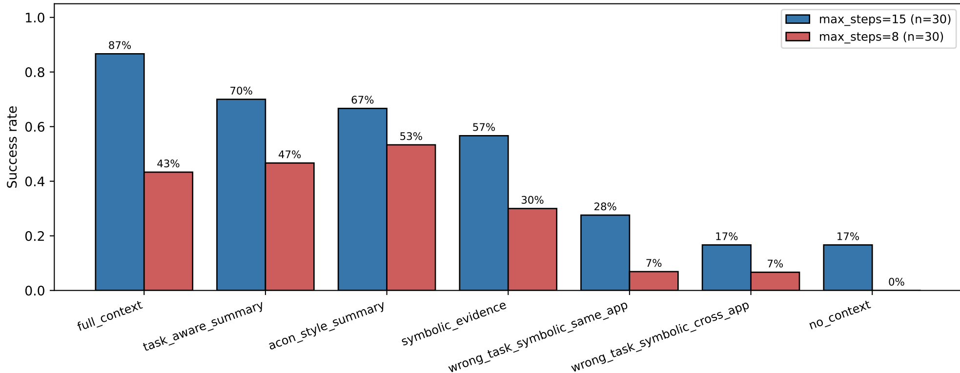
Behavioral utility: success under loose vs strict budget
