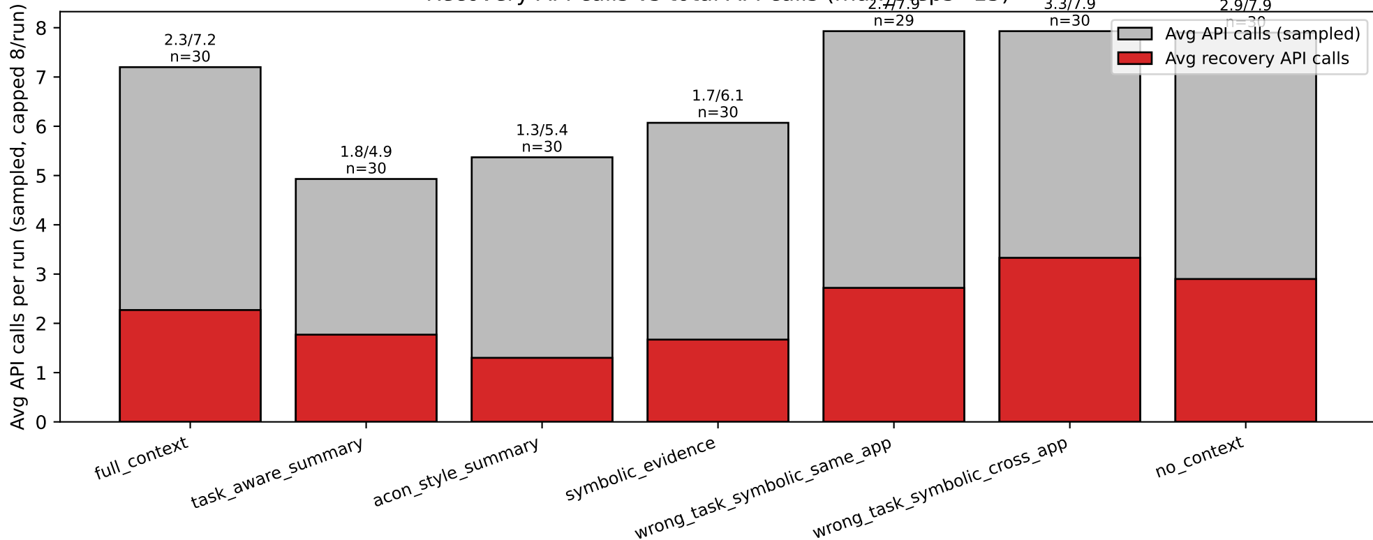
Recovery API calls vs total API calls (max_steps=15)
