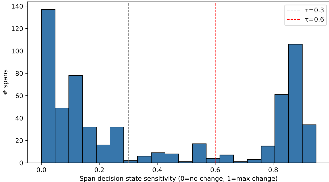
Distribution of span sensitivity scores (n=618 spans)
