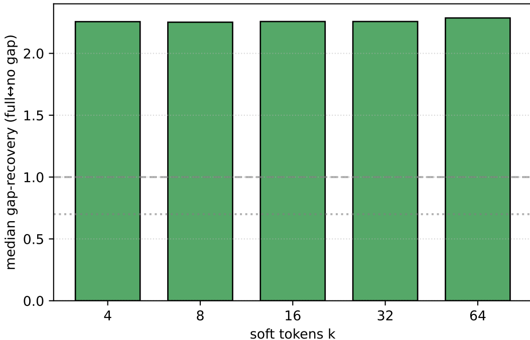
Soft-token oracle: gap recovery vs k
