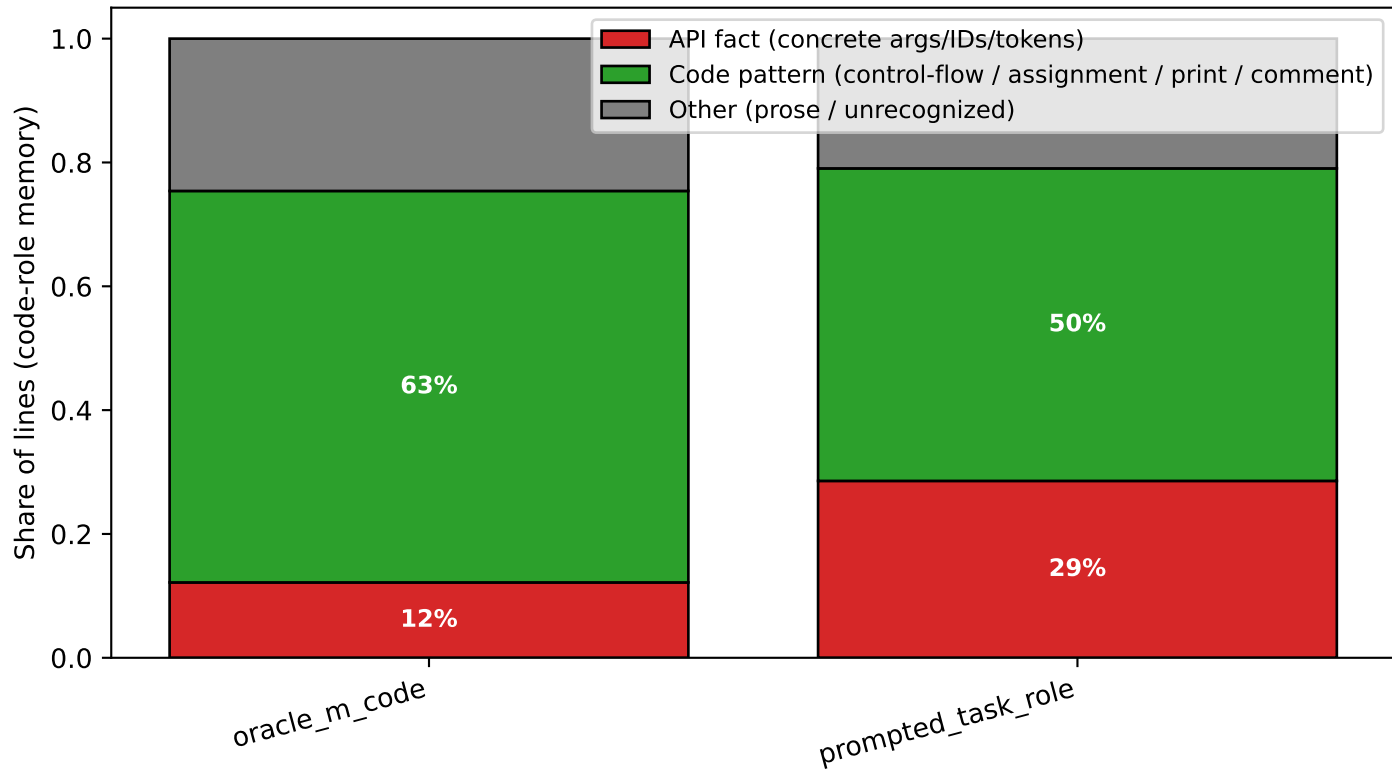
Code-role memory composition at B=512
