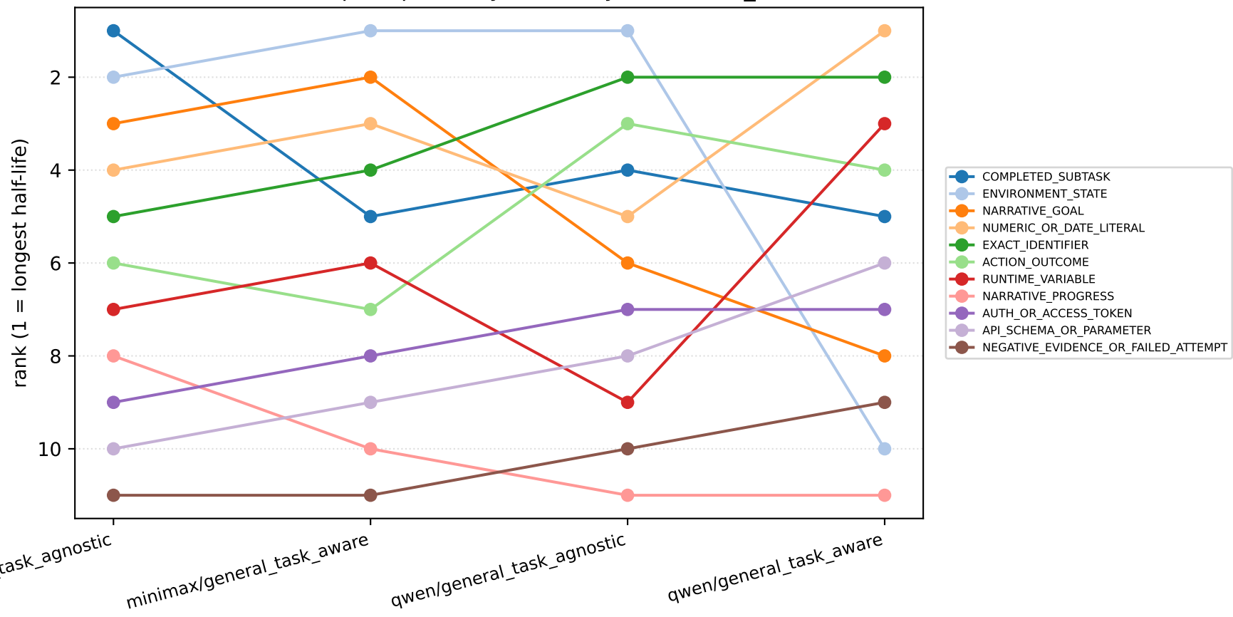
Cross model / prompt-family hierarchy rank (RAW_FULL)
