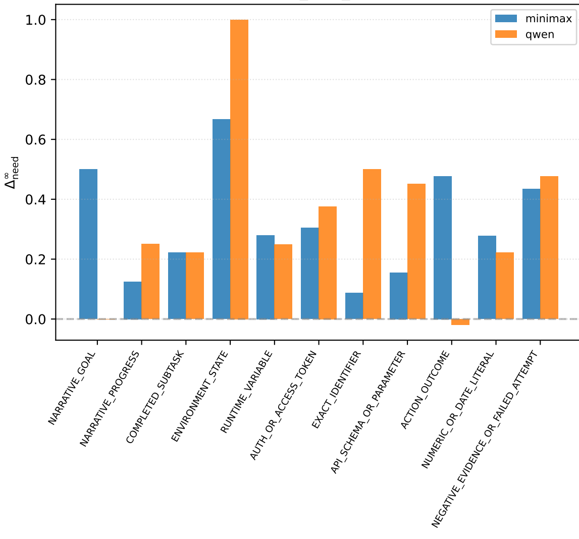
Fixed-point need shift by fact type general_task_aware
