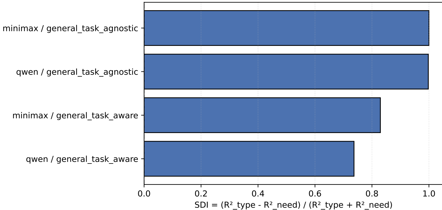
Surface Dominance — general prompts (v8)
