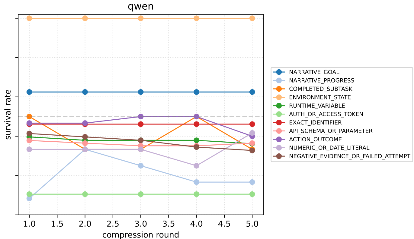
Iterative compression: survival by fact type
