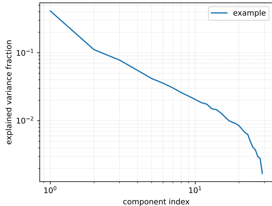
Example-level active subspace spectrum (layer 18)
