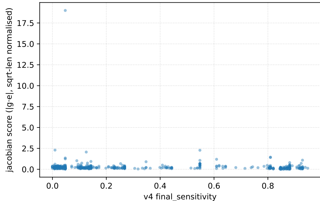
Jacobian vs v4 finite-difference (global Spearman=-0.200)
