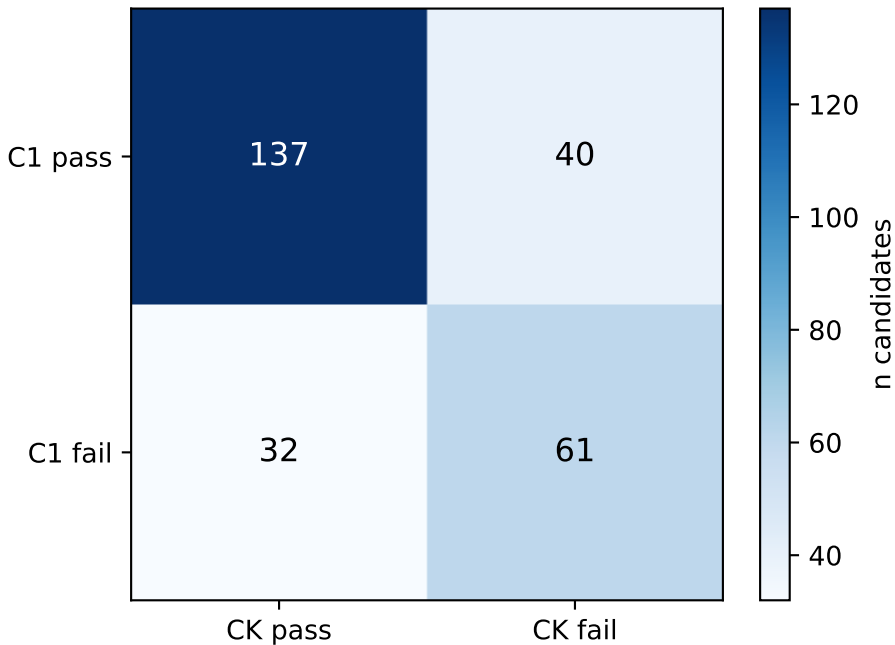
C1 vs CK transition matrix
