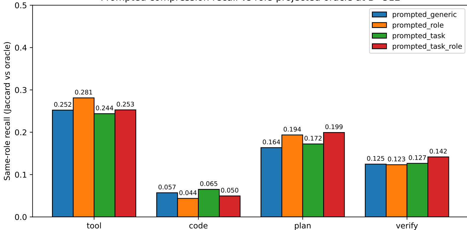
Prompted compression recall vs role-projected oracle at B=512
