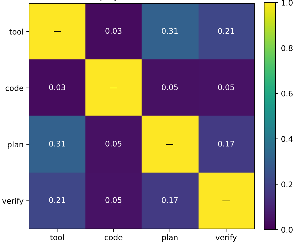
Oracle (role-projected) cross-role at B=512
