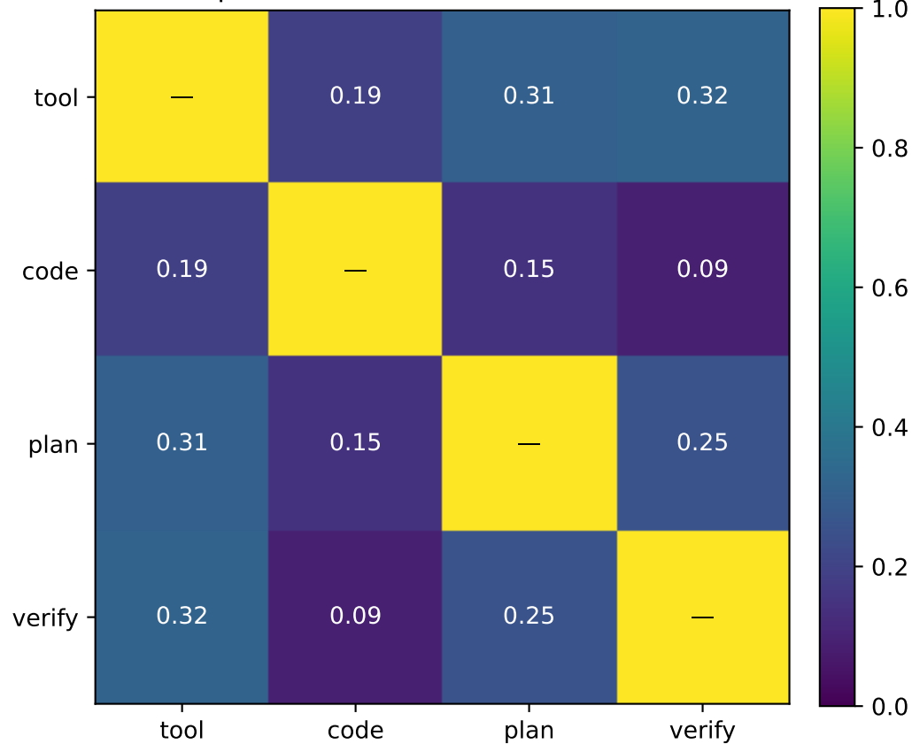
Prompted (task+role) cross-role at B=512
