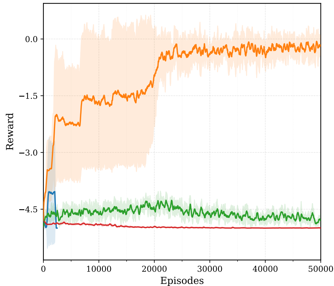
Gridworld
