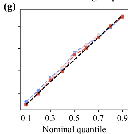
Heteroscedastic log-Laplace
