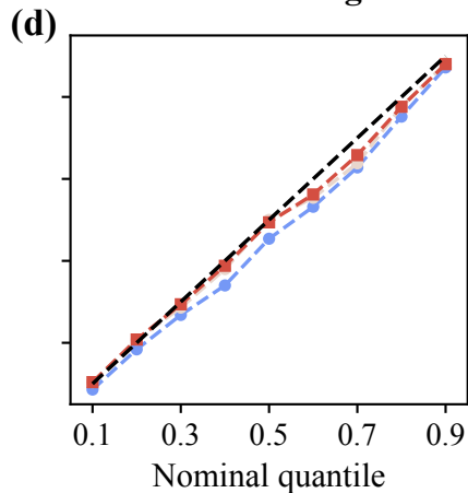
Heteroscedastic lognormal
