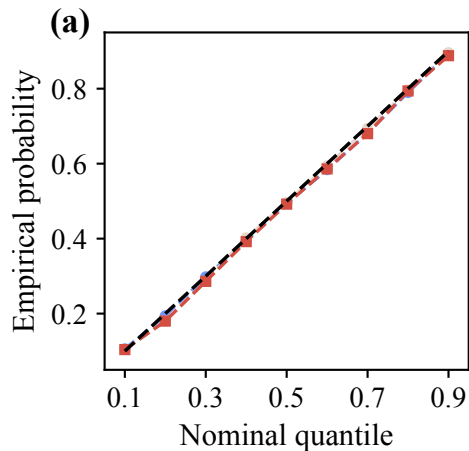
Homoscedastic Gaussian
