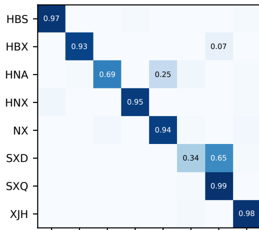
SNV-LR
