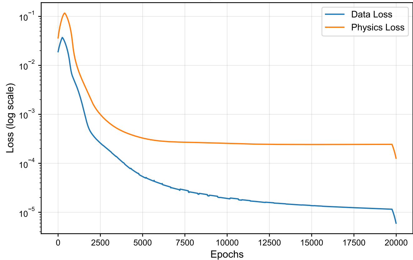
Training Loss Curves
