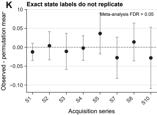
Figure S2. TCR repertoire structure, clone-state, and motif robustness | page 3 of 4
