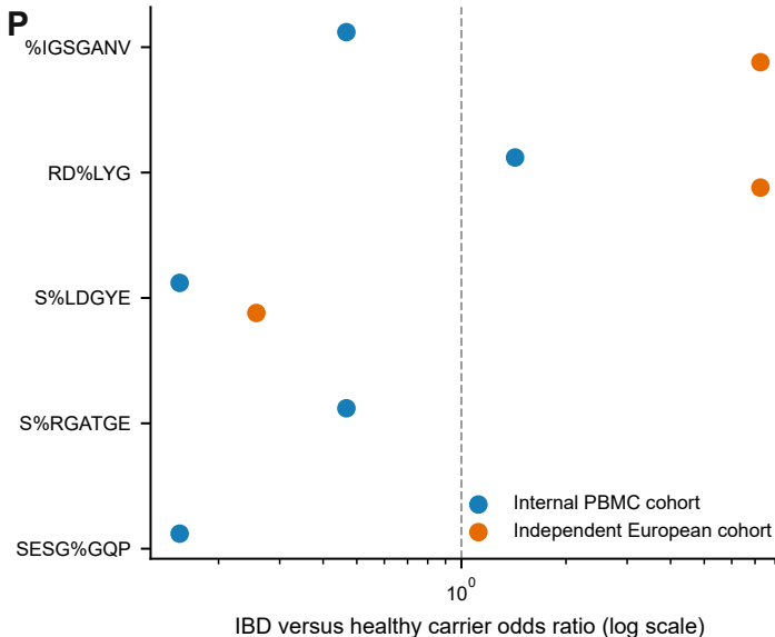
Figure S2. Independent motif context | page 4 of 4
