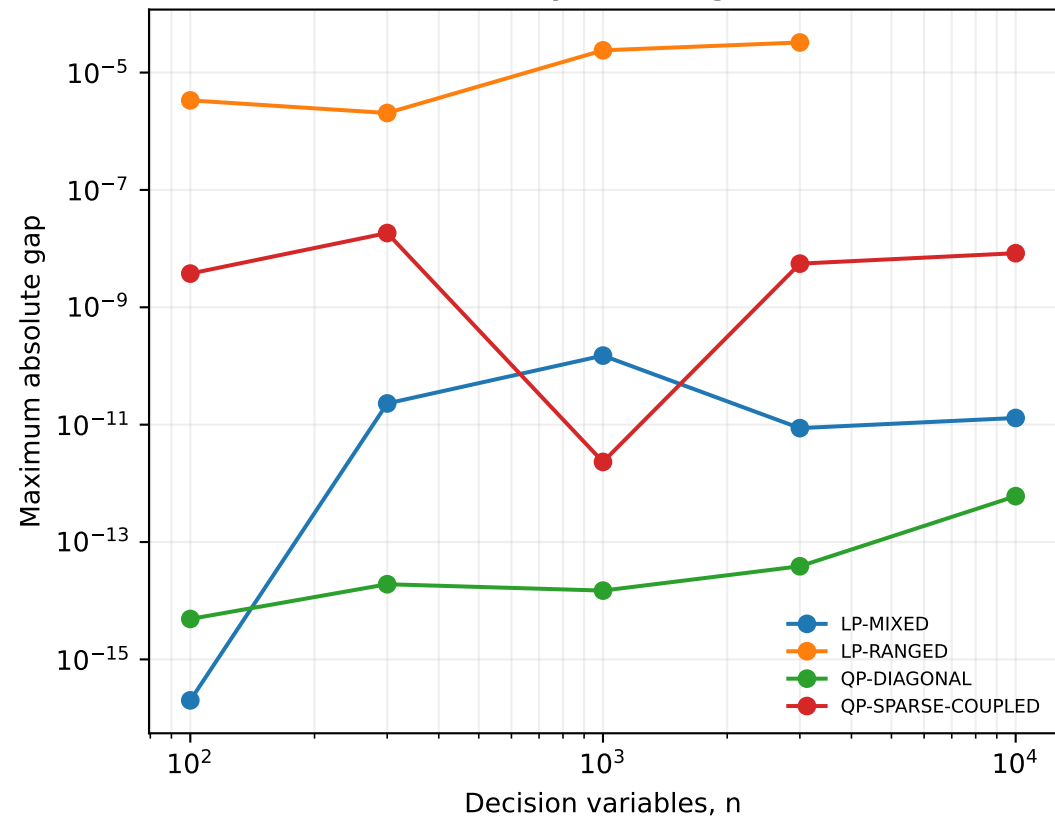
Canonical objective agreement
