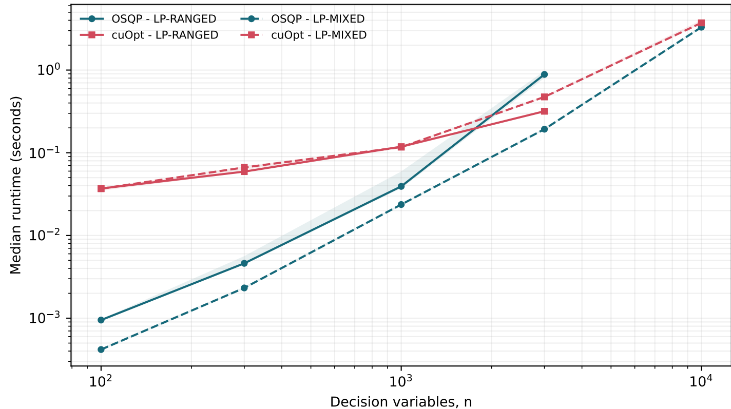
LP solve time versus n
