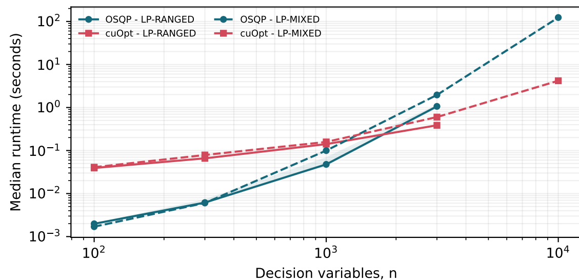
A. LP end-to-end runtime
