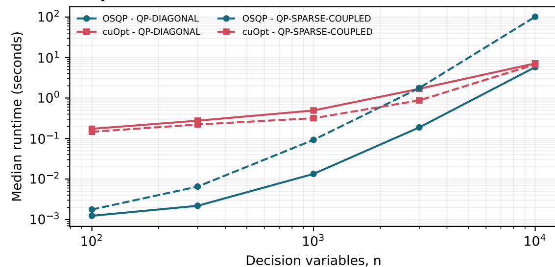
B. QP end-to-end runtime
