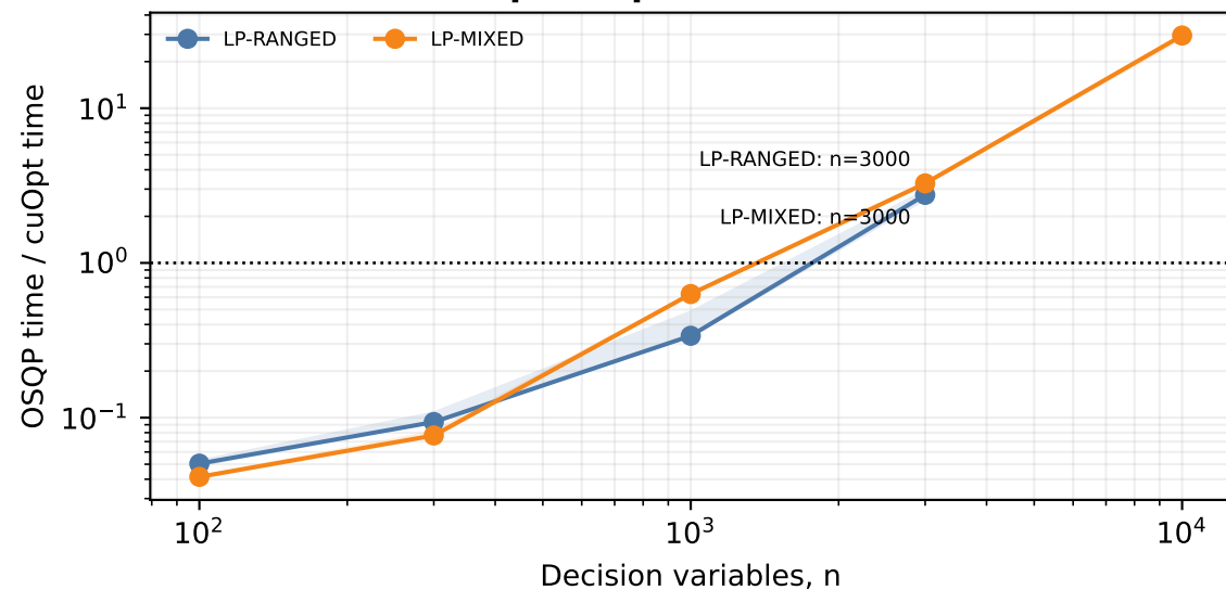
C. LP end-to-end speedup
