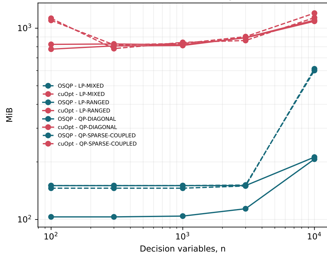
Peak host memory
