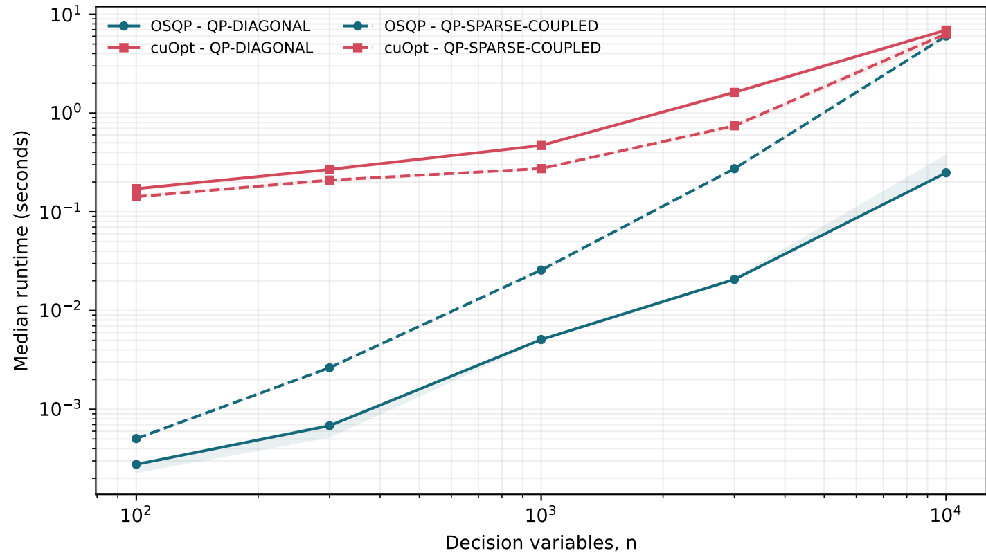
QP solve time versus n
