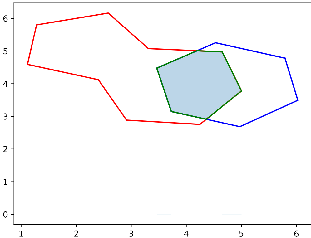
Contour of the overlap area (green) between two rings (blue and red)
