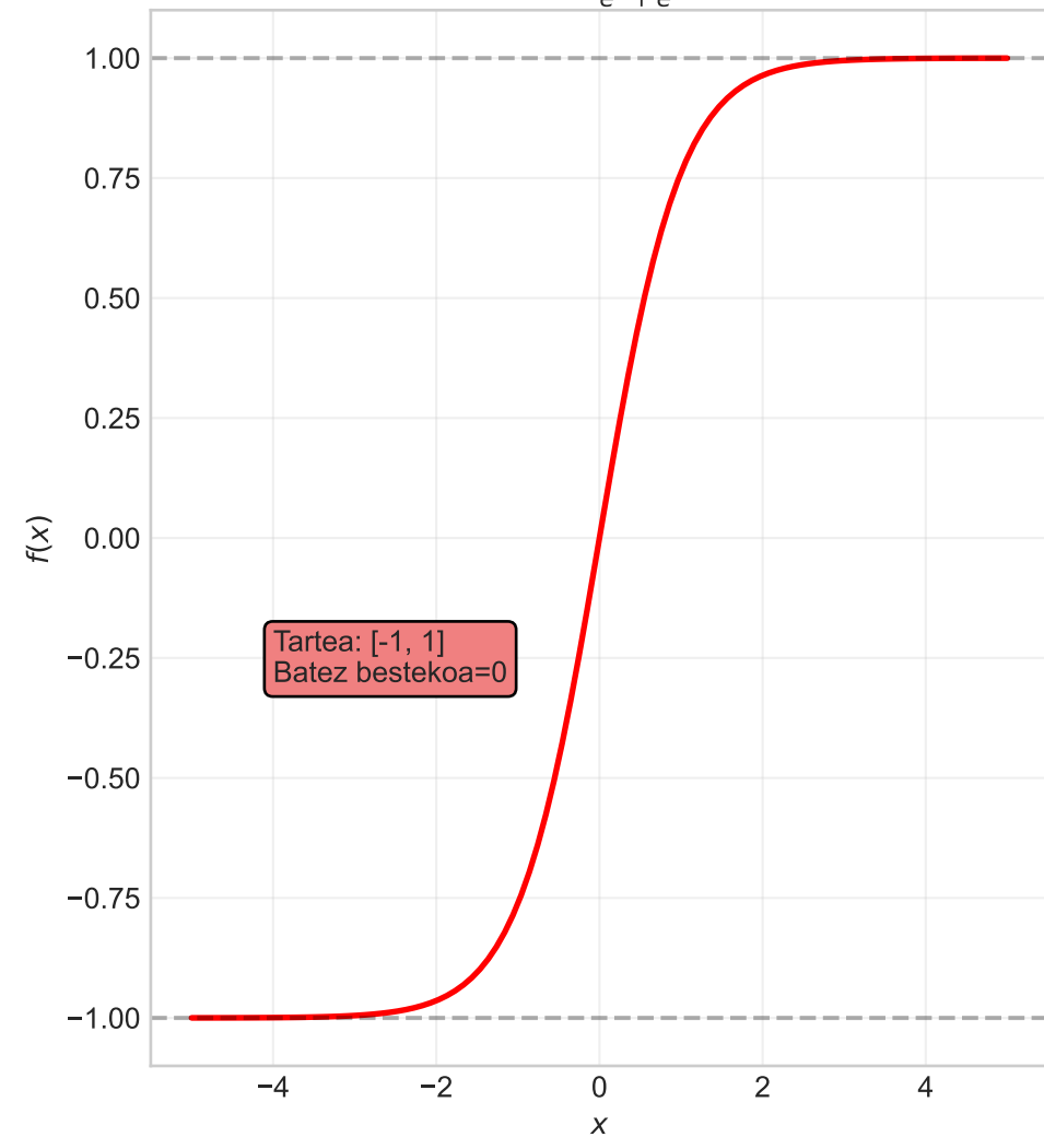
Tanh: \frac{e^x - e^{-x}}{e^x + e^{-x}}
