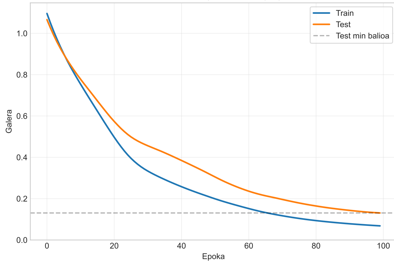
Sare Sinplea (1 Hidden Layer)
