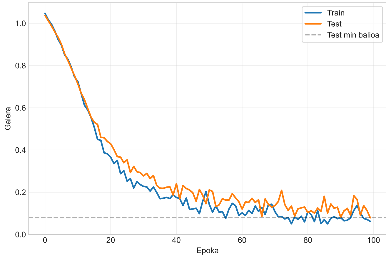
Sare Sakona (3 Hidden Layer)
