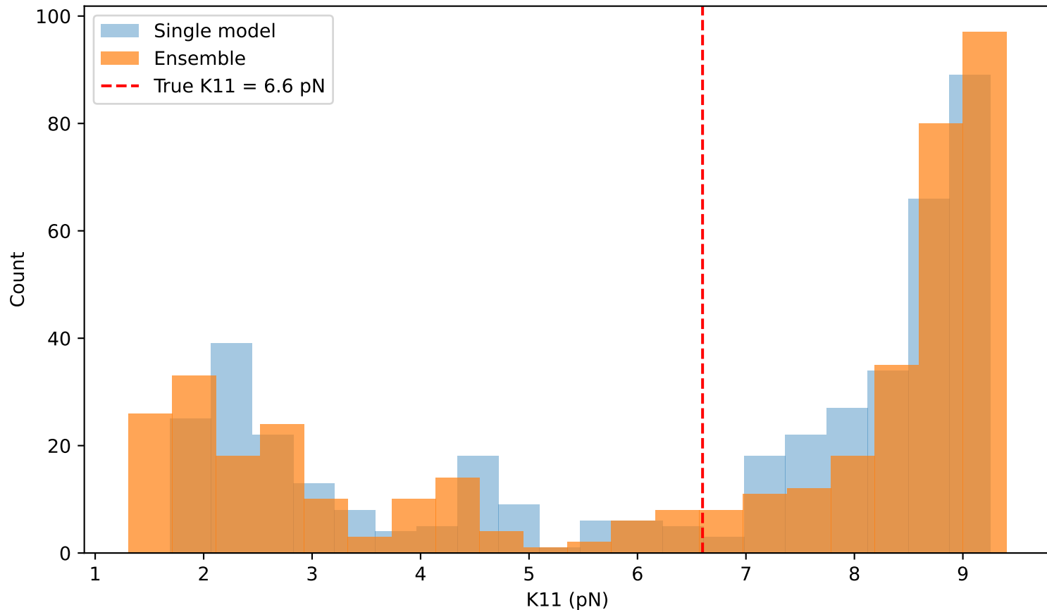
K11 Predictions: Single vs Ensemble
