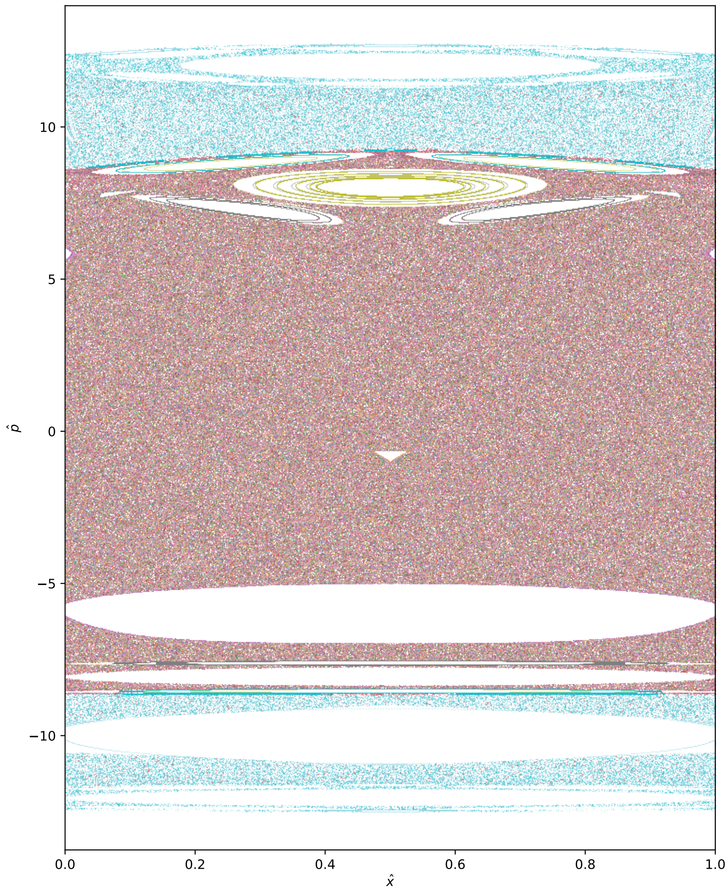
Phase portrait, k = 10 ( x_0 = 0.6122 )
