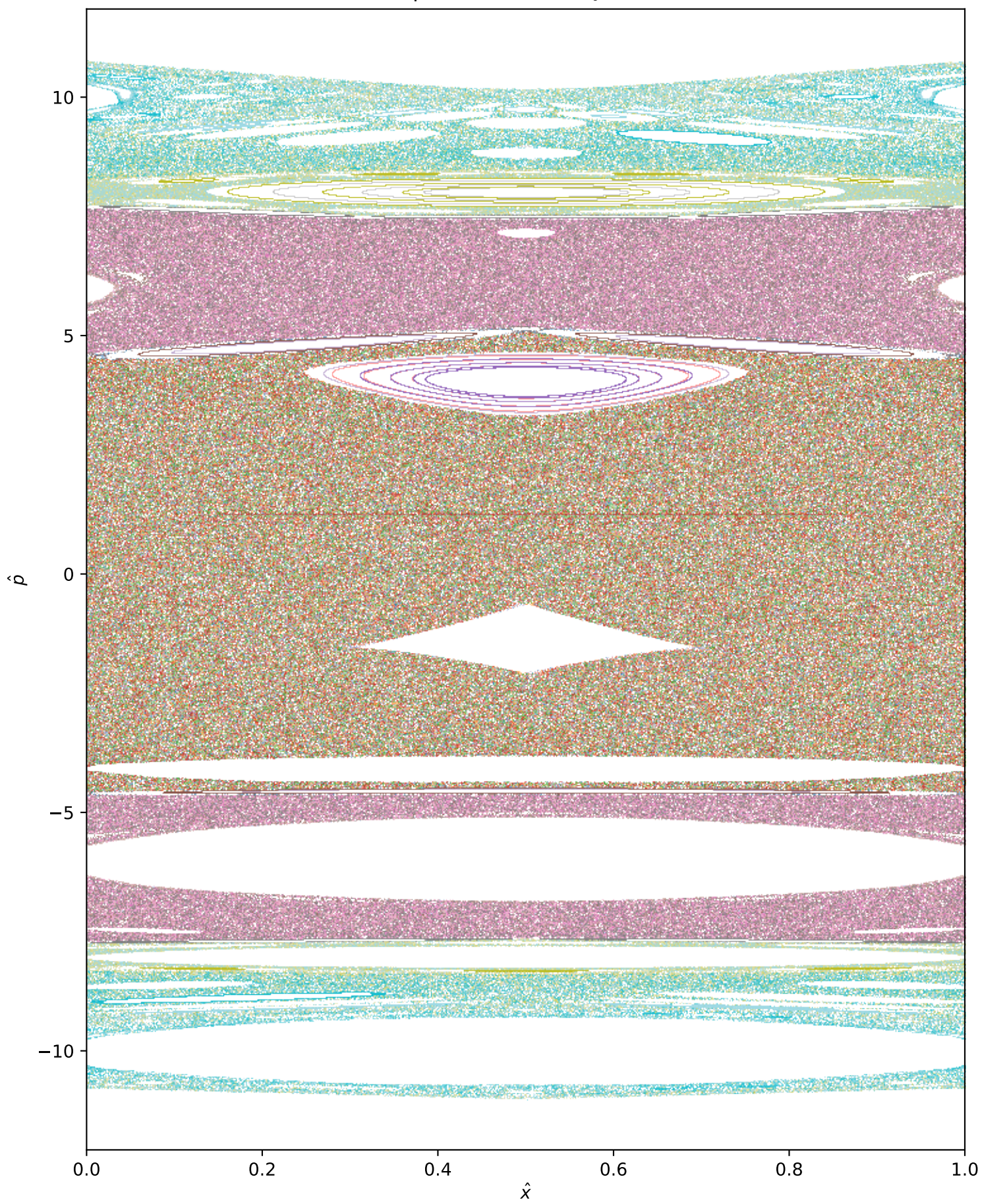
Phase portrait, k = 5 ( x_0 = 0.6122 )
