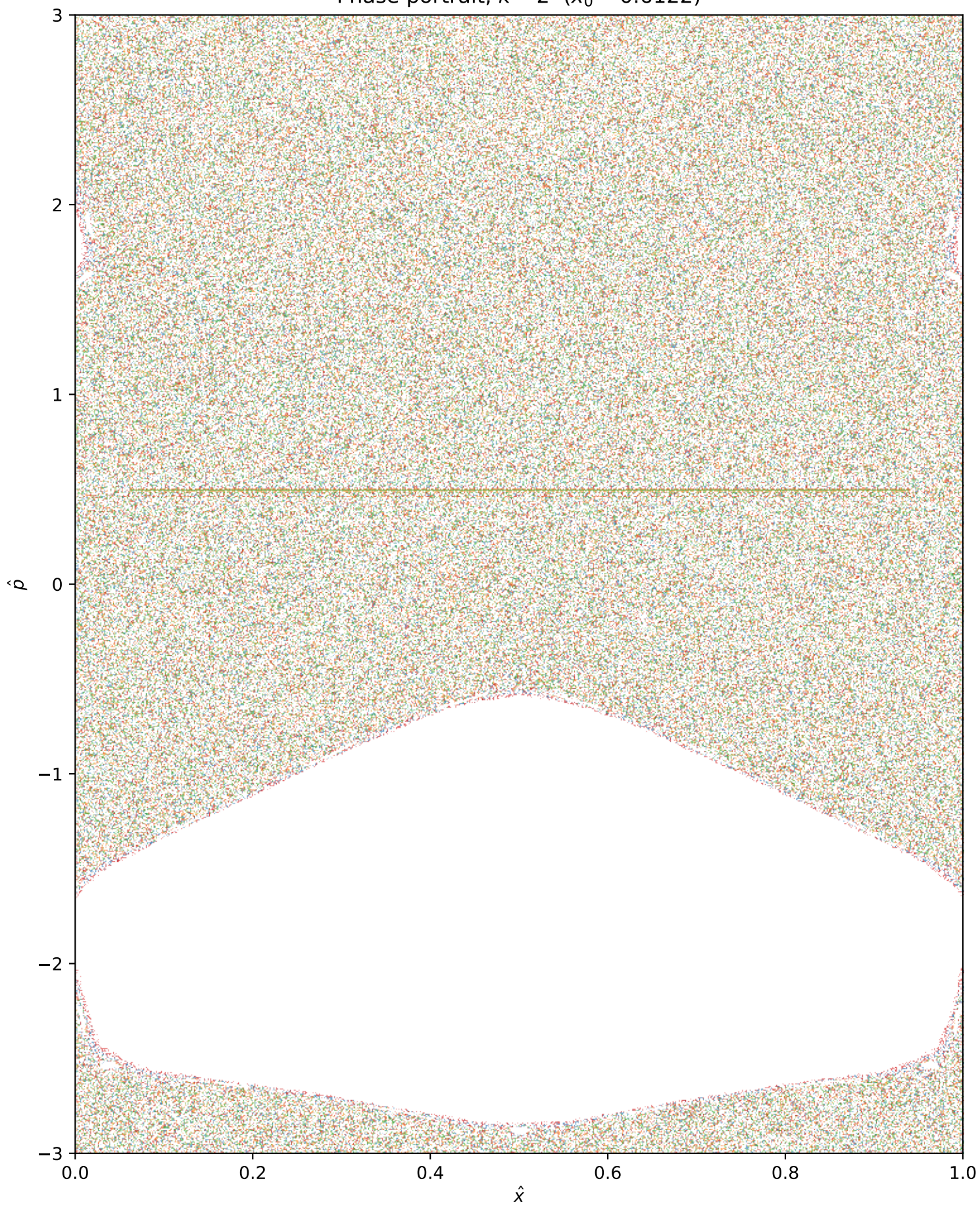
Phase portrait, k = 2 ( x_0 = 0.6122 )
